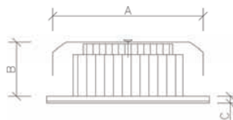
Retro fit 3 watt MR16 str. A-52mm cut out B- 25mm dybde C- 2,5mm tykk
